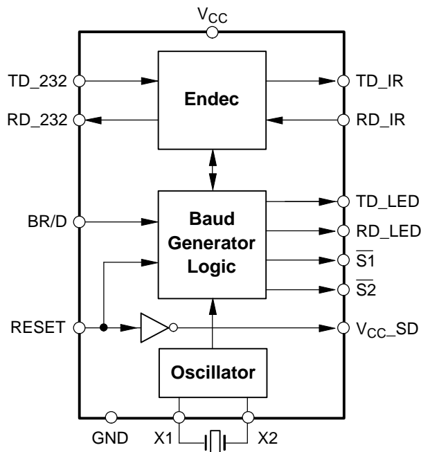
Figure 1. Block diagram
